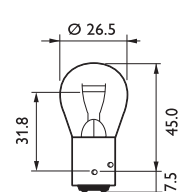
P21/4W
