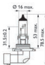
HB4
